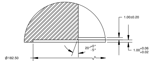
DETAIL - C
